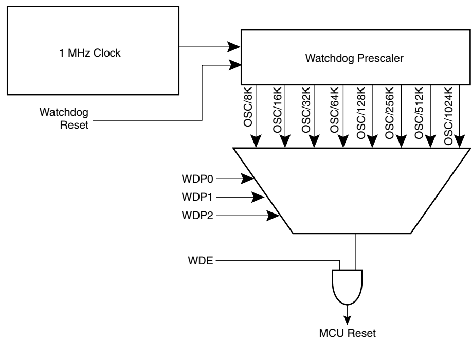
Figure 11. Watchdog Timer
