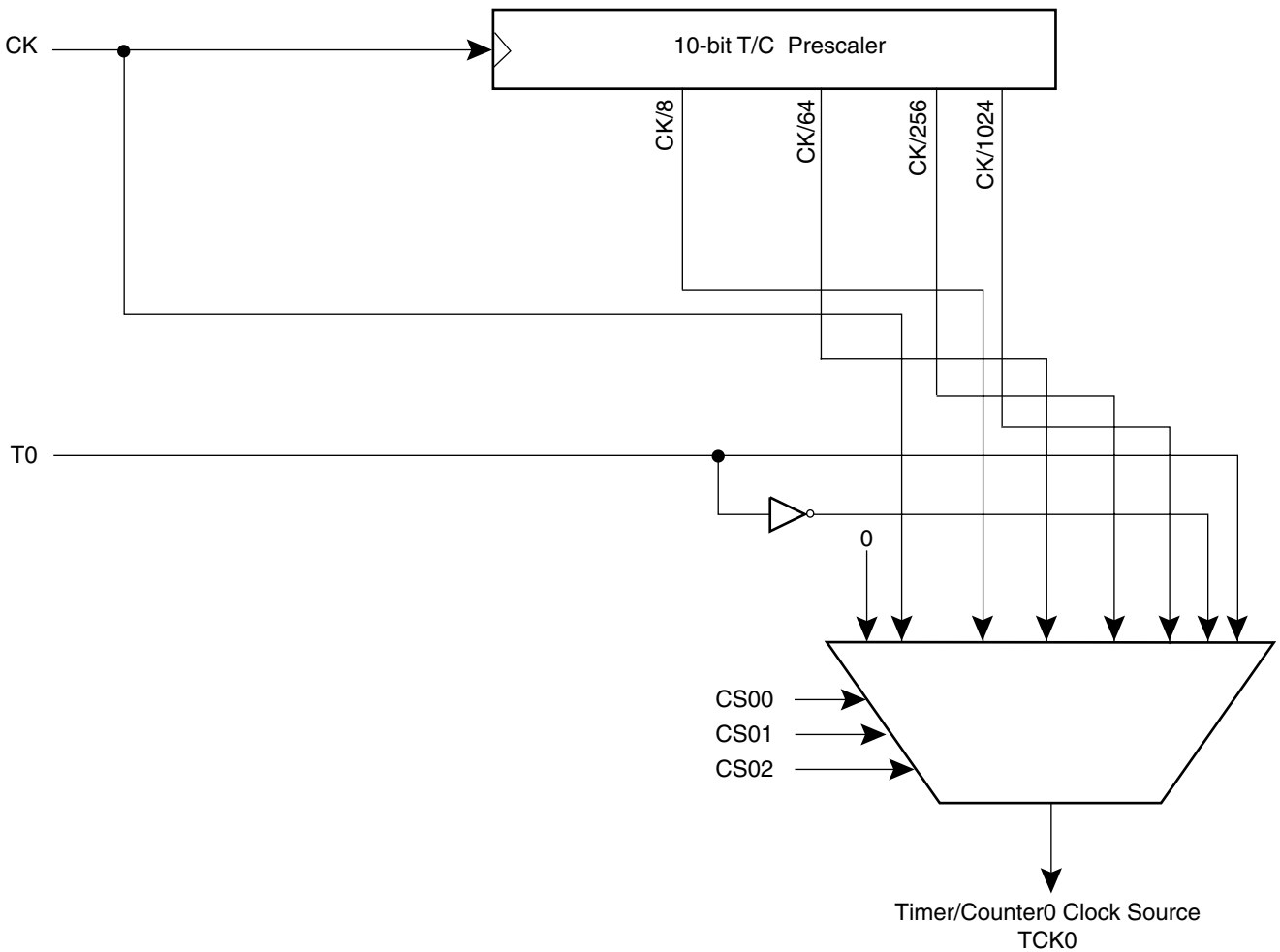
Figure 9. Timer/Counter Prescaler
